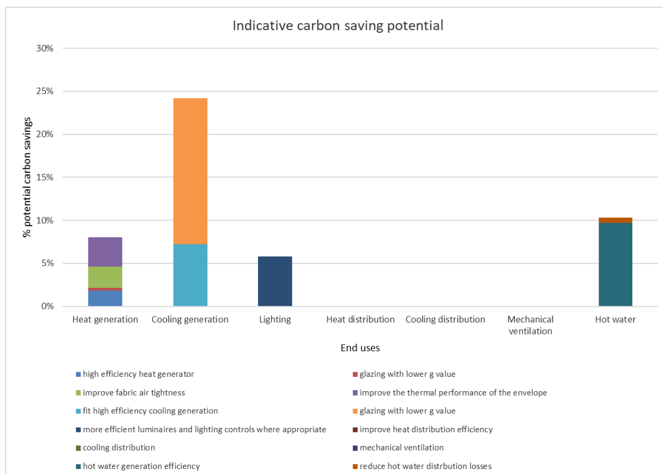
Figure 5: Example of output - Indicative carbon saving potential
