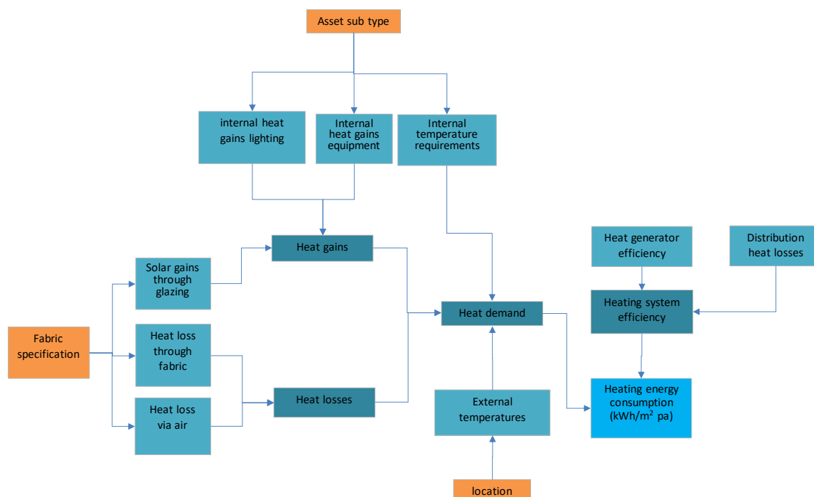
Figure 3: Schematic of the simplified energy modelling approach for space heating
