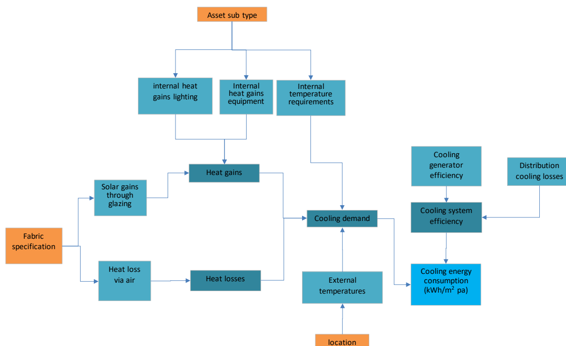
Figure 4: Schematic of the simplified energy modelling approach for space cooling
